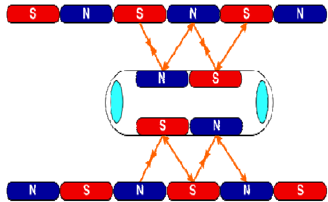
Figure 2: Propulsion
