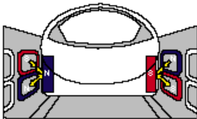
Figure 1: Levitation
