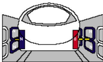
Figure 4: Guidance
