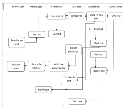
Figure. 4 Activity Diagram.
