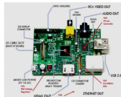
Fig. 6 : Raspberry pi card
