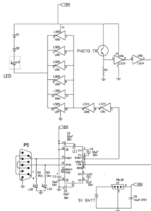
Figure 7: Li-Fi circuit diagram
