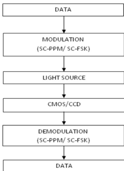
Figure 5: Six step process of data transmission using Li-Fi
