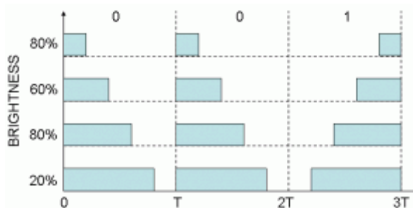
Figure 3: Variable Pulse Position Modulation to support dimming [4]
