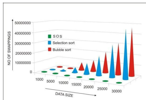
Fig. 2: Number of swapping operations vs. Data size
