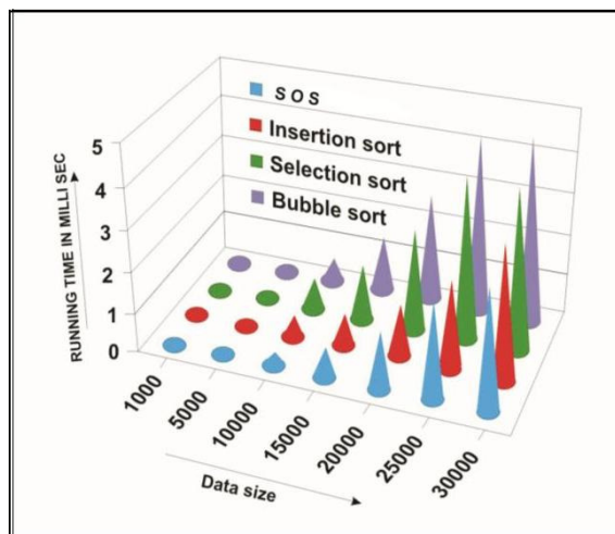
Fig. 1: Running time vs. Data size
